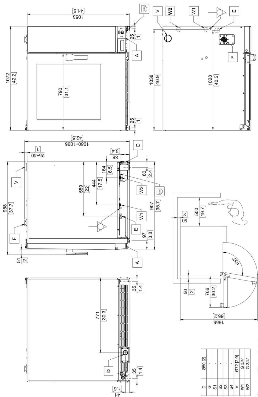
Dimensions: Millimeters [inches]
